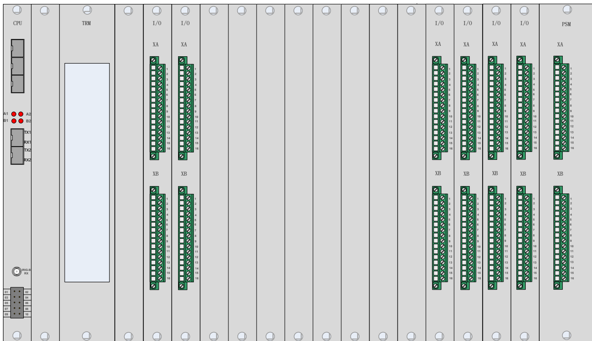
Figure 6.1.6 1/1 19" Case Rear Panel of this relay (Optical Ethernet)
