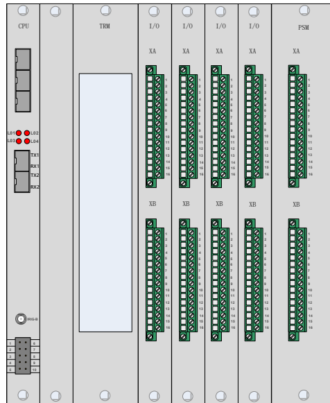
Figure 6.1.3 1/2 19" Case Rear Panel of this relay(Optical Ethernet)
