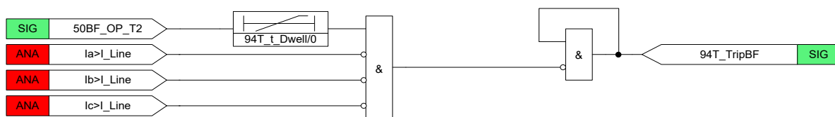
Figure 3.33.3 Logic Diagram of Tripping breaker failure
