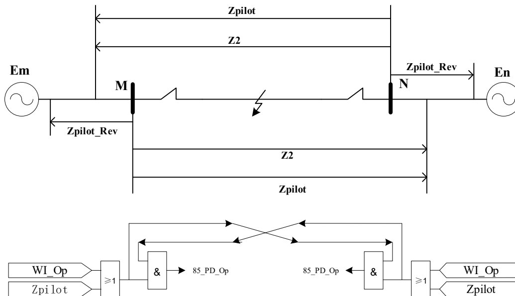
Figure 3.9.7 Simple schematic of POTT
