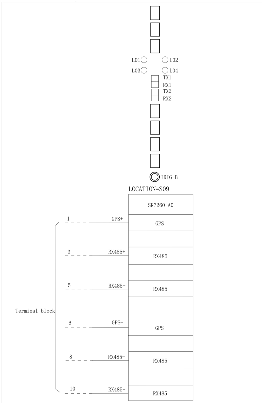
Figure 14.6.2 Communication interfaces
