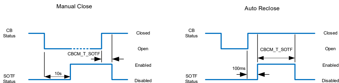
Figure 4.4.5 Logic diagram of automatic closing signal
