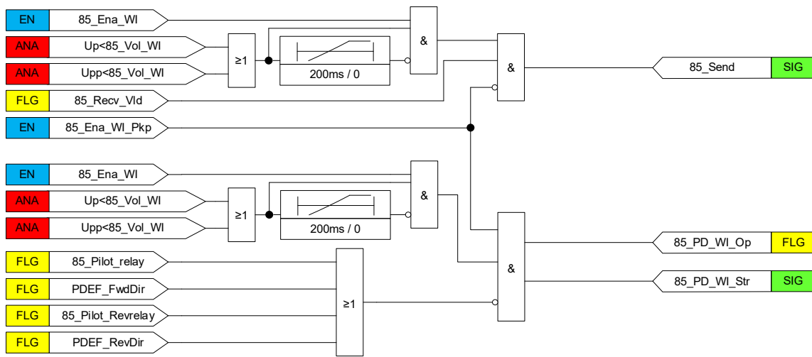
Figure 3.9.15 Weak infeed logic without pickup
