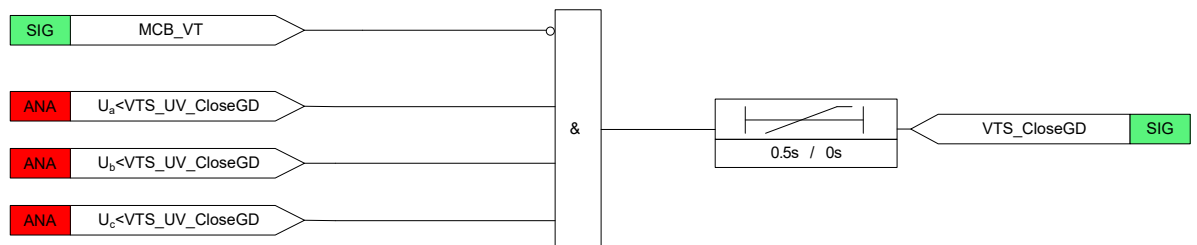
Figure 4.3.2 Logic Diagram of Permit closed gourd disconnector
