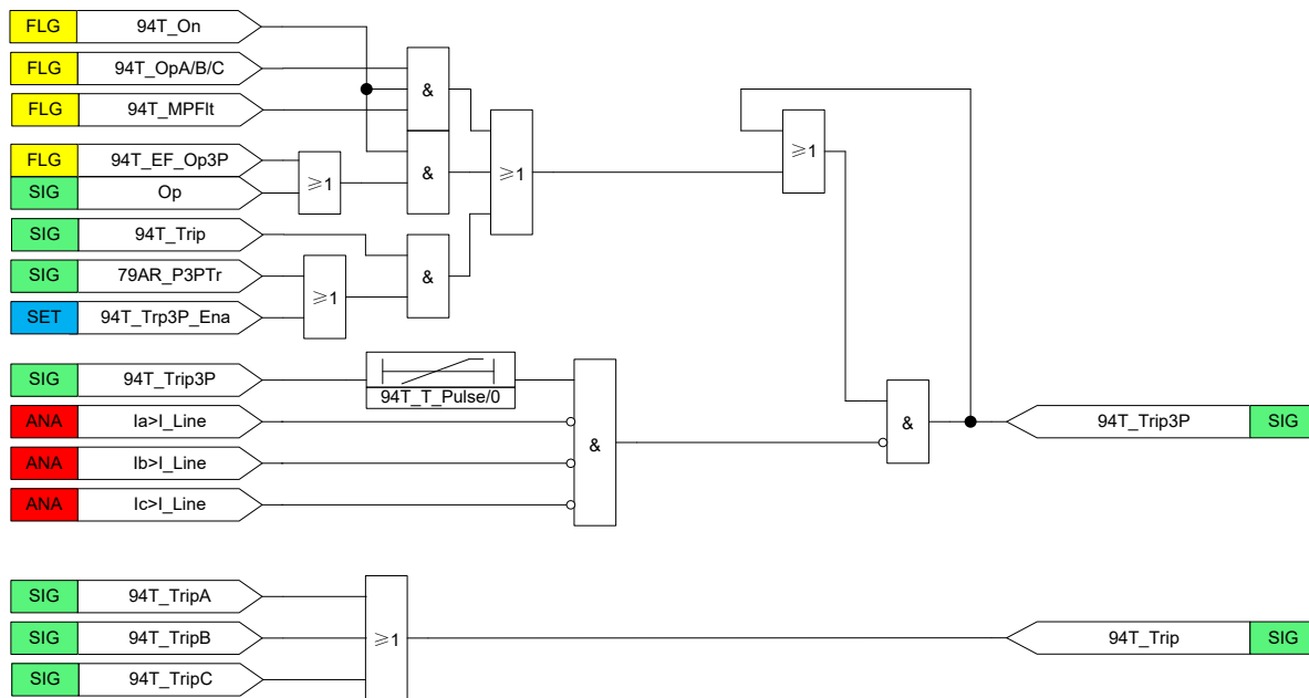
Figure 3.33.1 Logic Diagram of 94T
