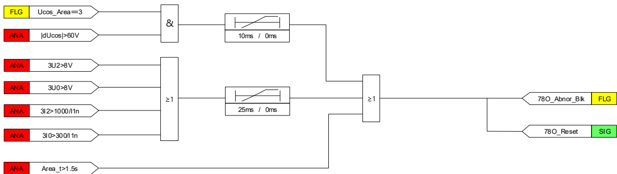
Figure 3.8.9 Abnormal Condition Blocking of 780
