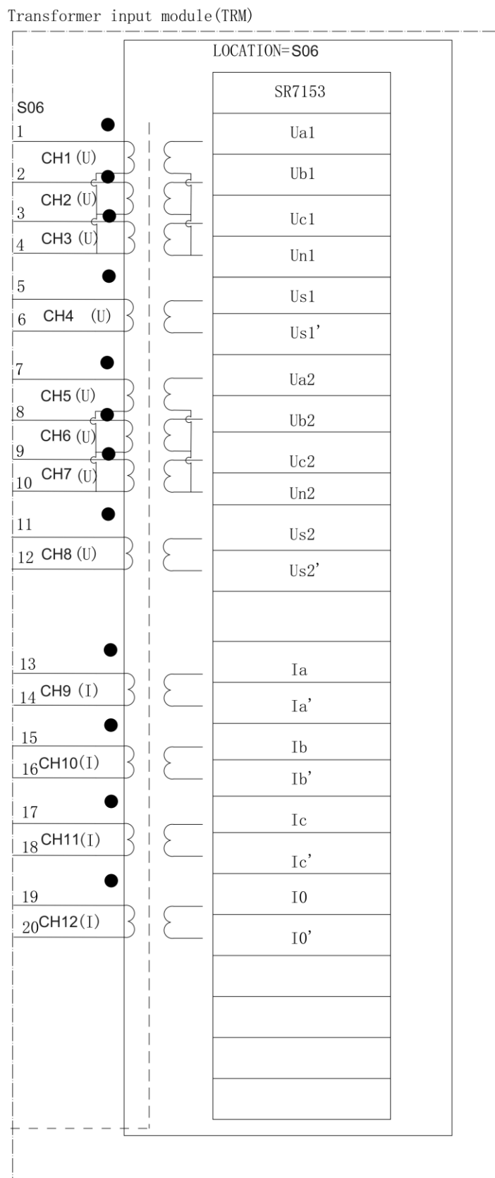
Figure 14.2.3-2 Transformer input module: SR7153-CQ(8VT+4CT)
