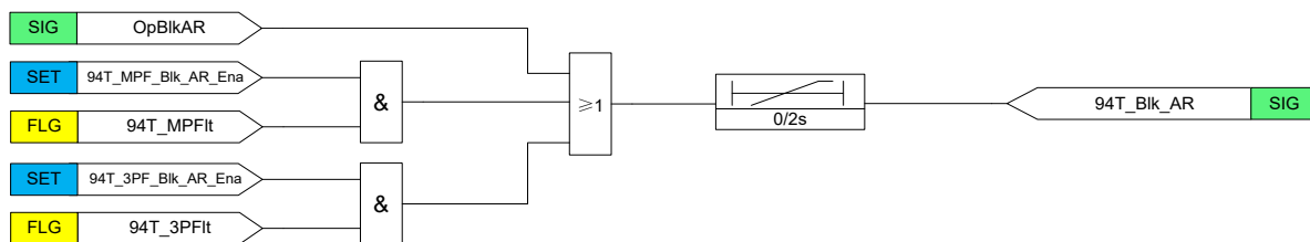
Figure 3.33.2 Logic Diagram of Blocking AR
