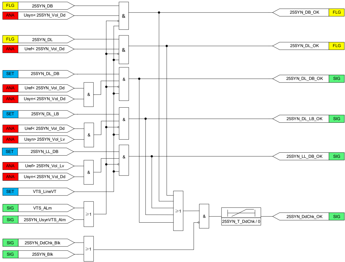
Figure 3.30.2 Logic Diagram of Dead charge check logic (the logic setting VTS_LineVT is set to “1”)
