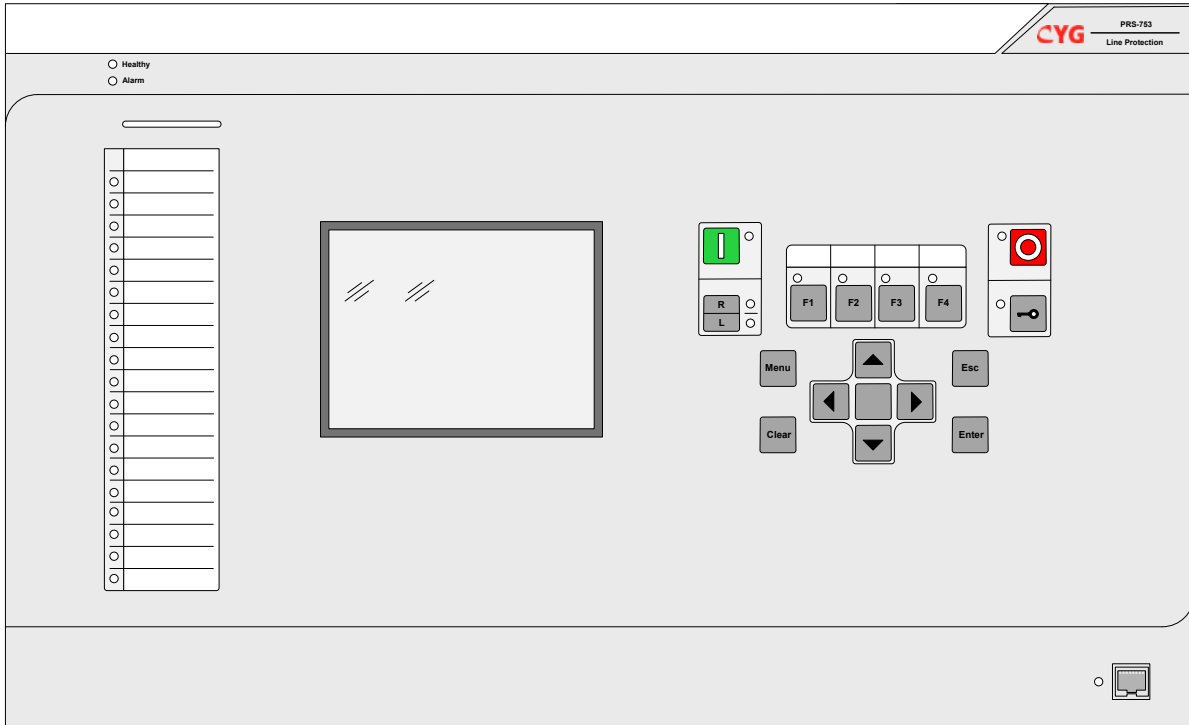
Figure 6.1.5 1/1 19" Case Front Panel of this relay
