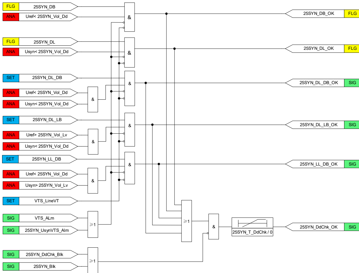
Figure 3.30.1 Logic Diagram of Dead charge check logic (the logic setting VTS_LineVT is set to “0”)
