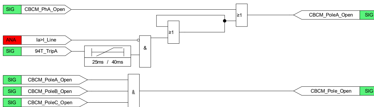
Figure 4.4.2 Logic diagram of pole open state (phase A)
