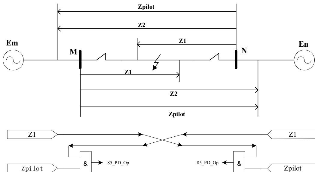
Figure 3.9.5 Simple schematic of PUTT
