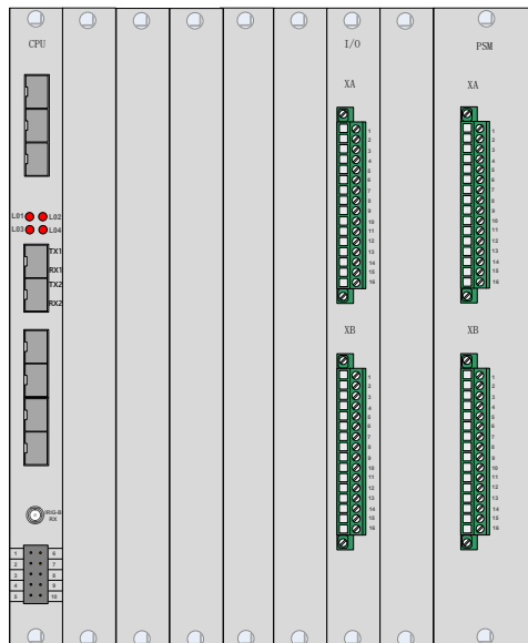
Figure 6.1.4 1/2 19" Case Rear Panel of this relay (Process Level)
