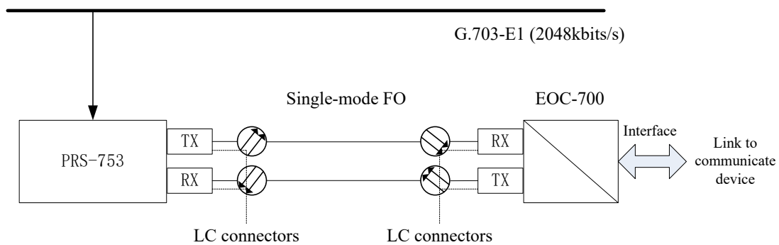
Figure 3.6.2 Connect to a communication network via EOC-700
