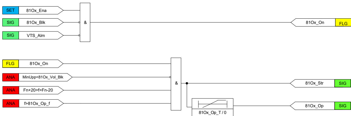
Figure 3.27.1 Logic Diagram of 81O
